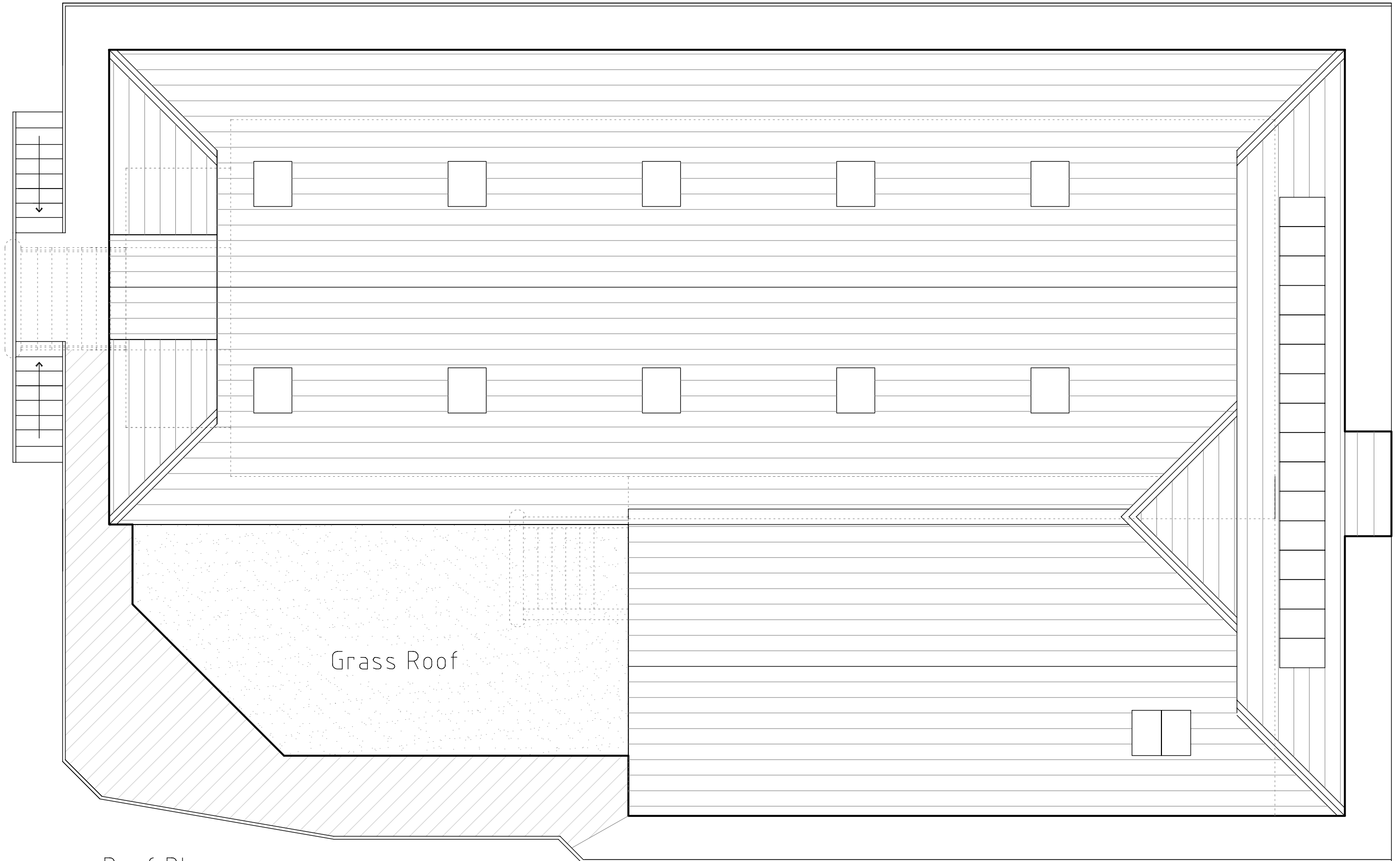
Roof Plan 1:100sc
